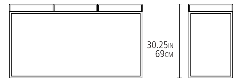
ELEVATIONS
